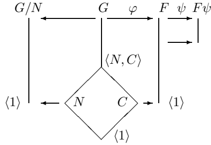
FIGURE 1. Structure of an extension with non-abelian kernel
