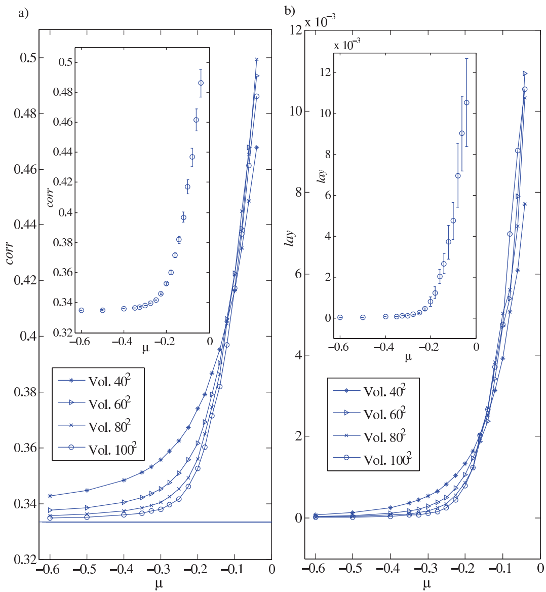
Fig. 4: (Color online) Data from the 1 : \infty model. a) Correlation vs. \mu , for volumes 40^2 through 100^2 , where the horizontal line represents corr = 1/3 ; b) layer size vs. \mu , for volumes 40^2 through 100^2 . Error bars in both insets represent 95% confidence intervals for volume 100^2 , and for low \mu are smaller than the data circles.
