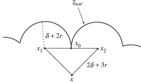
FIGURE 3: Pictured are x_1, x_2 \in \Psi(\omega') \subset W_\gamma and x \in \Psi(\omega \cap W_\gamma) , but x \notin \Psi(\omega') . For such x , d(x, \gamma) > \sqrt{5r^2 + 8r\delta + 3\delta^2} . This can be seen in the above picture, in which the distance from x to \gamma is minimized by placing x_1 and x_2 as far apart as possible.
