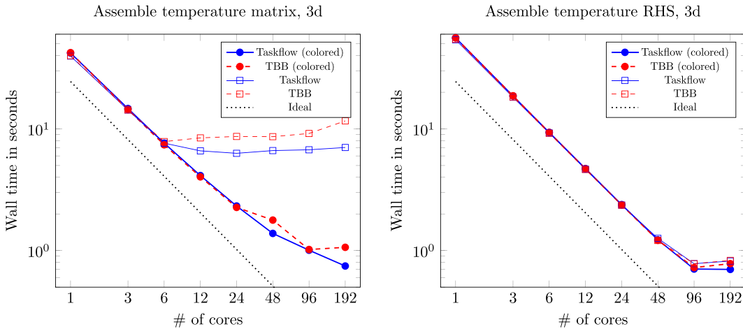
Figure 1: Assembly times in a modified step-32 (left: temperature matrix assembly, right: temperature right-hand side assembly) comparing TBB and Taskflow with and without coloring. These figures correspond to the middle row of [8, Fig. 4]. Lines with squares match “Implementation 2” in [8]; the lines with circles labeled “colored” match “Implementation 3” therein.
