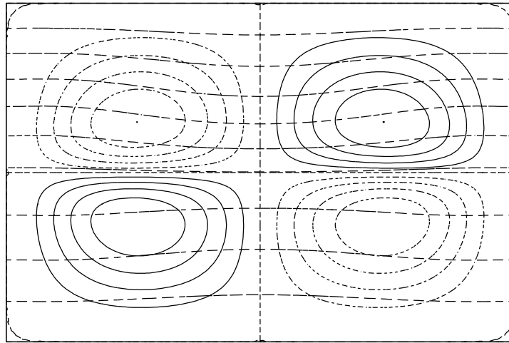
FIG. 4. Streamlines and isotherms when heating from above for the connected two-cell flow at Ma=2100 and contact angle 89.89 degrees. (Point A, figure 3.) Solid lines indicate positive values of the streamfunction (anti-clockwise circulation) and dashed lines indicate negative values of the streamfunction (clockwise circulation). Pr = 4.38, Ca = 2.5 \times 10^{-6}, \rho_r = 0.844, \mu_r = 0.812, \alpha_r = 1.0, c_r = 1.02, k_r = 0.638, v_r = 1.0, \lambda = 1.5 .
