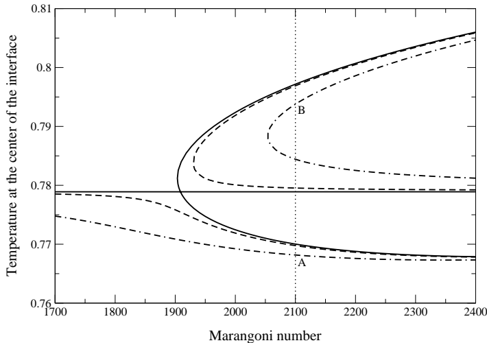
FIG. 3. Bifurcation diagram near instability to two-cell flows when heating from above for contact angles equal to 90 (solid line), 89.99 (dashed line) and 89.89 (chained line) degrees. Pr = 4.38 , Ca = 2.5 \times 10^{-6} , \rho_r = 0.844 , \mu_r = 0.812 , \alpha_r = 1.0 , c_r = 1.02 , k_r = 0.638 , v_r = 1.0 , \lambda = 1.5 .
