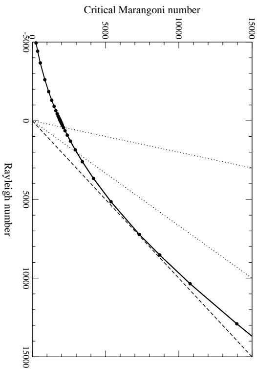
FIG. 11. Effect of buoyancy on bifurcation to two-cell flows when heating from above.
