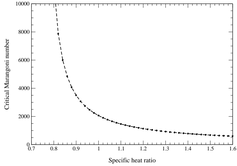
FIG. 7. Effect of specific heat ratio on bifurcation to two-cell flows when heating from above.
