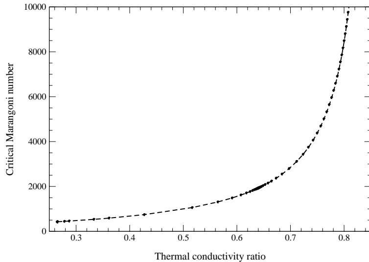
FIG. 10. Effect of conductivity ratio on bifurcation to two-cell flows when heating from above. Pr = 4.38 , Ca = 2.5 \times 10^{-6} , \rho_r = 0.844 , \mu_r = 0.812 , \alpha_r = 1.0 , c_r = 1.02 , v_r = 1.0 , \lambda = 1.5 .
