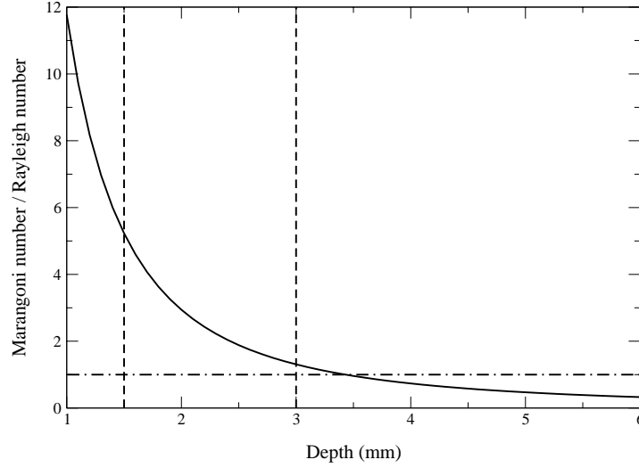
FIG. 12. Ratio of Marangoni number to Rayleigh number as a function of depth.
