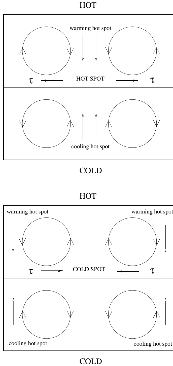
FIG. 6. Thermocapillary instability mechanism when heating from above.
