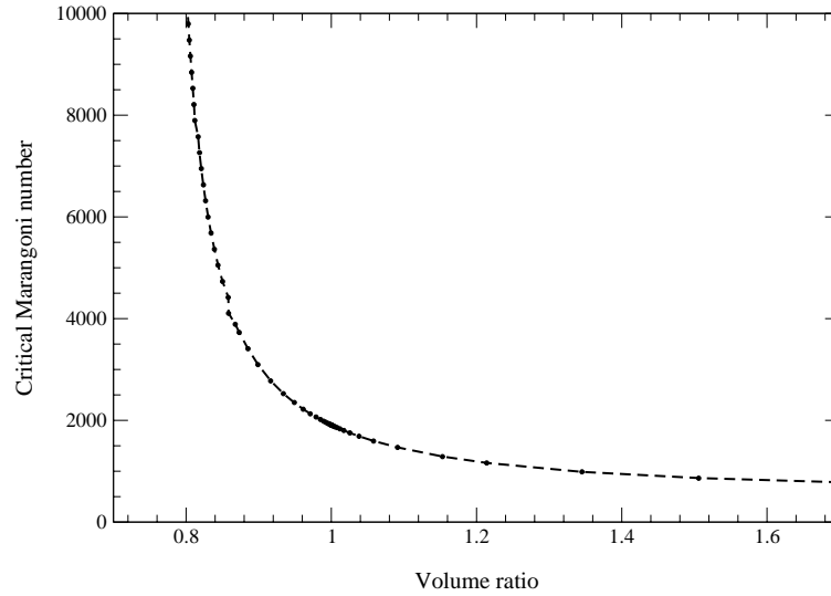
FIG. 9. Effect of volume ratio on bifurcation to two-cell flows when heating from above.
