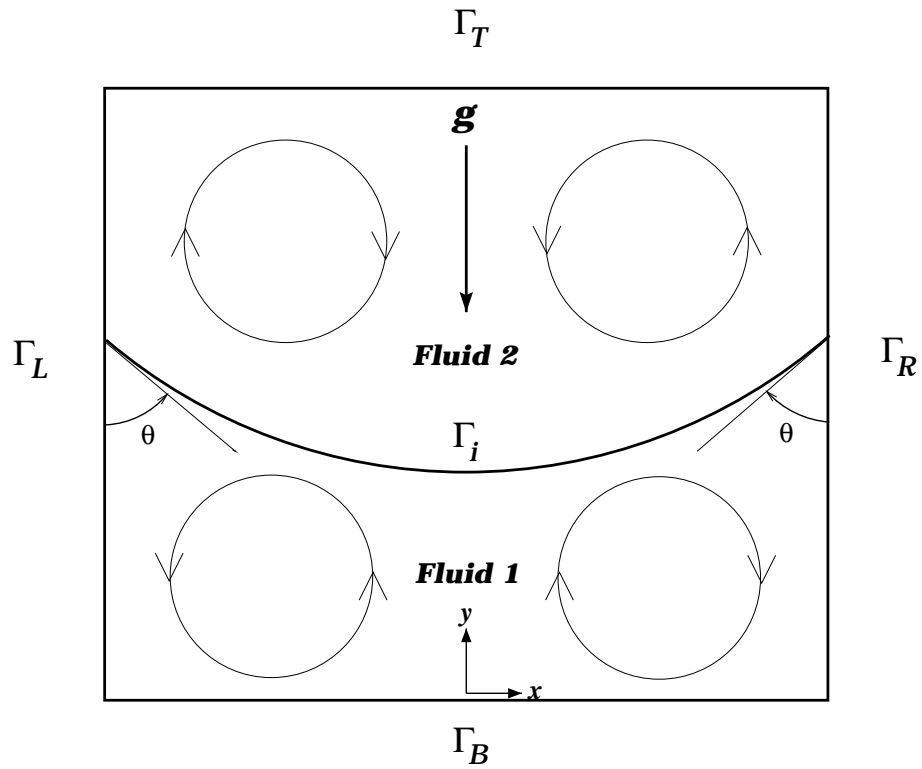
FIG. 1. Sketch of the physical domain
