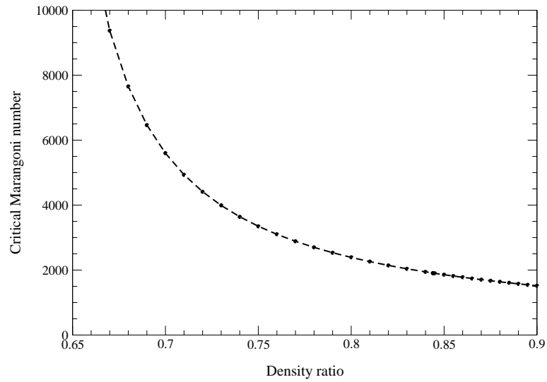
FIG. 8. Effect of density ratio on bifurcation to two-cell flows when heating from above.
