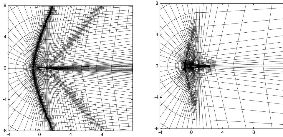
Fig. 8. Supersonic compressible flow at M = 1.2 , \text{Re} = 1000 , \alpha = 0^\circ around the NACA0012 airfoil: Residual-based refined mesh of 17,670 elements with 282,720 degrees of freedom and |J_{c_{dp}}(\mathbf{u}) - J_{c_{dp}}(\mathbf{u}_h)| = 1.9 \cdot 10^{-3} (left); goal-oriented (adjoint-based) refined mesh for c_{dp} : mesh of 10,038 elements with 160,608 degrees of freedom and |J_{c_{dp}}(\mathbf{u}) - J_{c_{dp}}(\mathbf{u}_h)| = 1.6 \cdot 10^{-4} (right).
