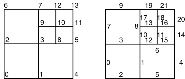
Fig. 4. Depictions of global enumerations of degrees of freedom on the mesh shown in Figure 2 for \mathbb{Q}_1 elements with degrees of freedom associated with vertices (left) and lowest order Nedelec elements with degrees of freedom on cell faces (right).
