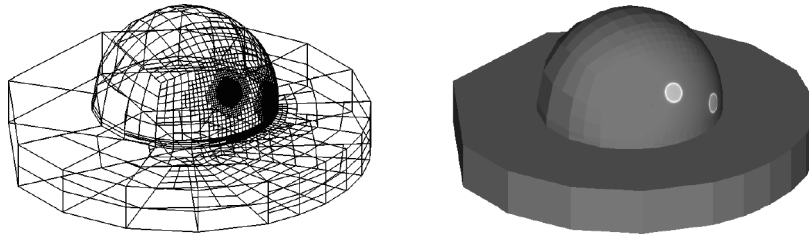
Fig. 9. Surface of a three-dimensional mesh with 66,989 cells simulating light propagation in a breast phantom geometry (left). Solution obtained on this mesh with 321,264 degrees of freedom (right).
