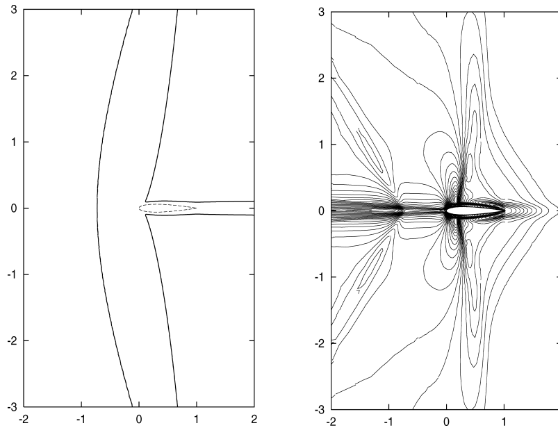
Fig. 7. Compressible flow at M = 1.2 , Re = 1000 , \alpha = 0^\circ around the NACA0012 airfoil: Sonic isolines of the flow solution (left); isolines of the first component of the computed adjoint solution (right).
