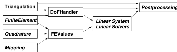
Fig. 1. An overview of the collaboration between the most important classes in deal.II. Abstract base classes and groups of classes are shown in italics. The discussion in this article roughly follows this figure from left to right.
