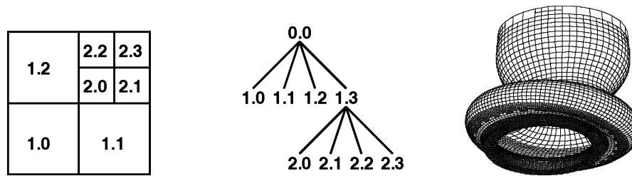
Fig. 2. A simple two-dimensional mesh with cells numbered based on their refinement level and index within a level (left) and the corresponding quad-tree of cells (middle). A complex three-dimensional mesh (right).
