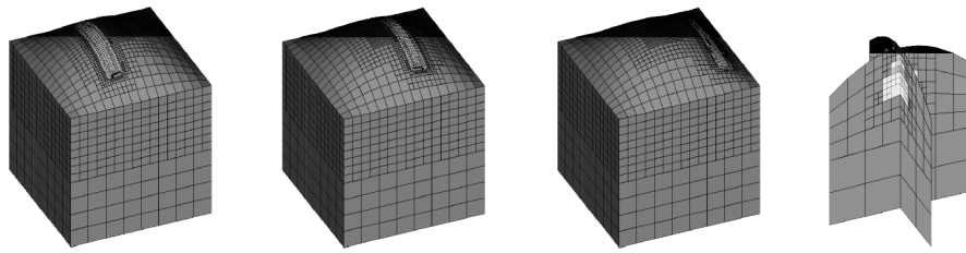
Fig. 10. Simulation of a widened laser scanning over a surface (left to center right). Cut planes through reconstructed tumor densities (right). Computations involved solving a PDE-constrained optimization problem with 640,902 unknowns.
