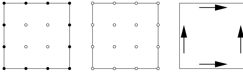
Fig. 3. Degrees of freedom of the standard (left) and discontinuous \mathbb{Q}_3 elements (middle), as well as lowest-order Nedelec elements (right). Filled circles indicate node functionals requiring continuity across a face, open circles have no such requirements. Arrows denote continuity only of the indicated vector component.
