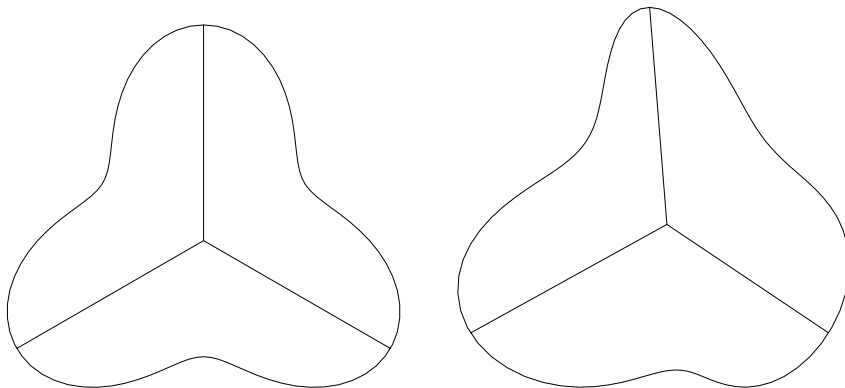
Figure 3: D_3 -Symmetric and Nearly D_3 -Symmetric Domain
