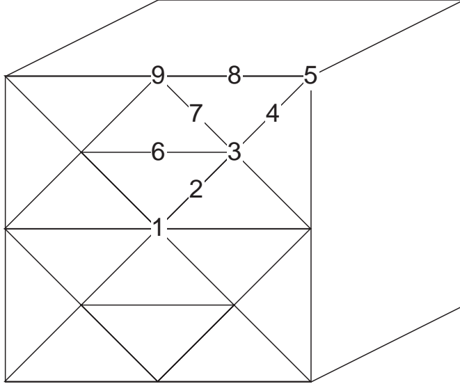
Figure 2: Cubical Surface with Collocation Points
