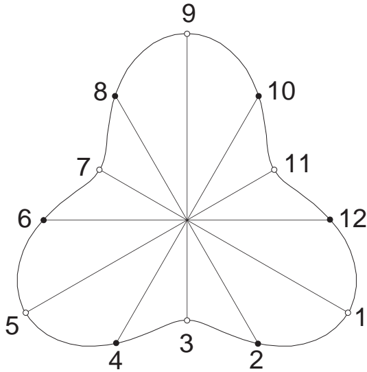
Figure 1: Domain with a D_3 -symmetry
